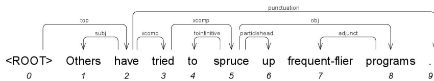
Figure 3: Dependency representation of the example sentence
