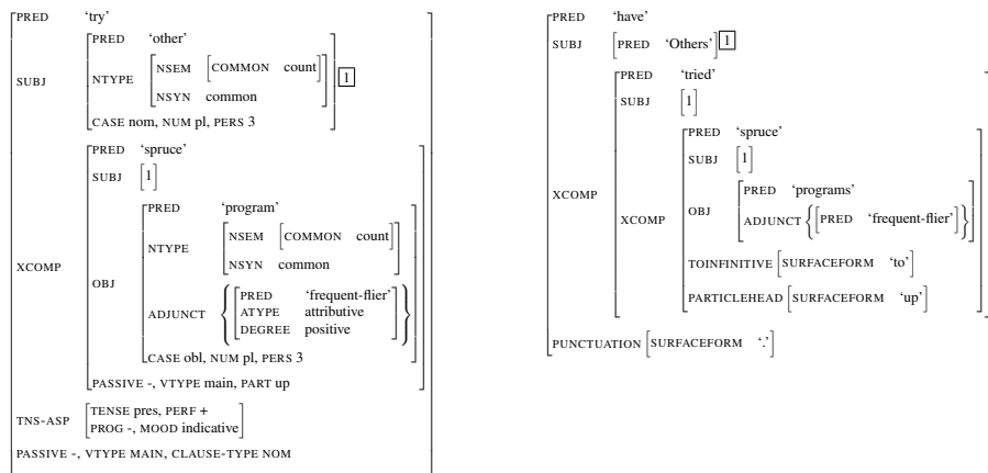
Figure 1: LFG f-structure for Others have tried to spruce up frequent-flier programs. in the original form (left) and as bilexical dependencies (right)
